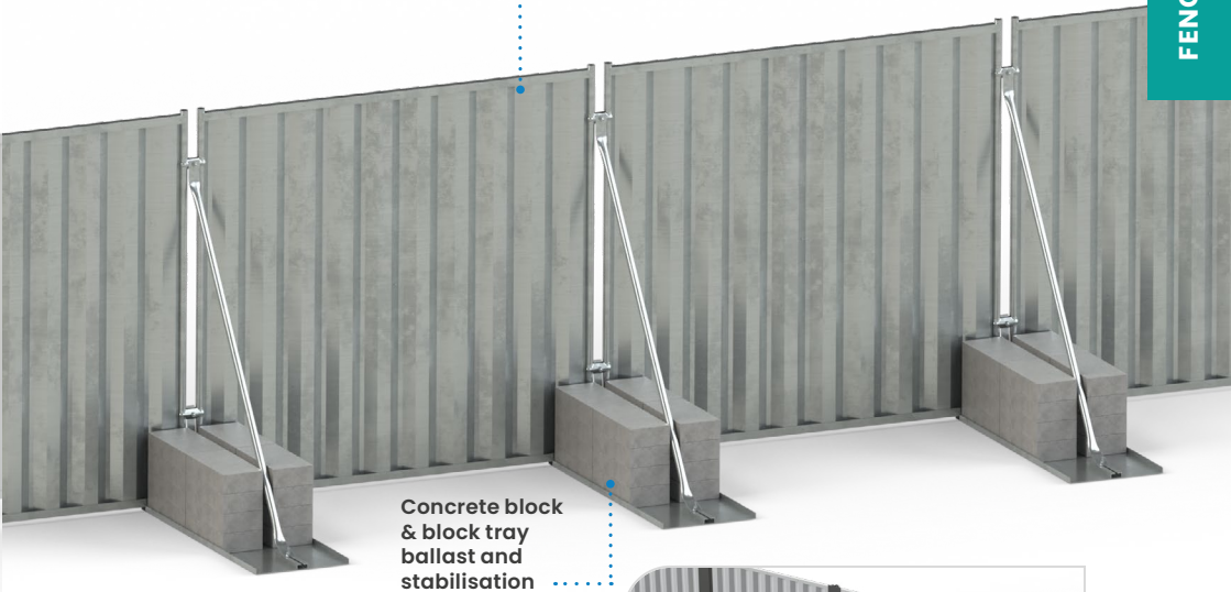
In / On Ground Hoarding Panel
